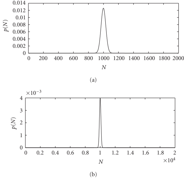
FIGURE 4: The probability mass function for Poisson distributions. (a): \lambda = 1000 ; (b): \lambda = 10000 .
