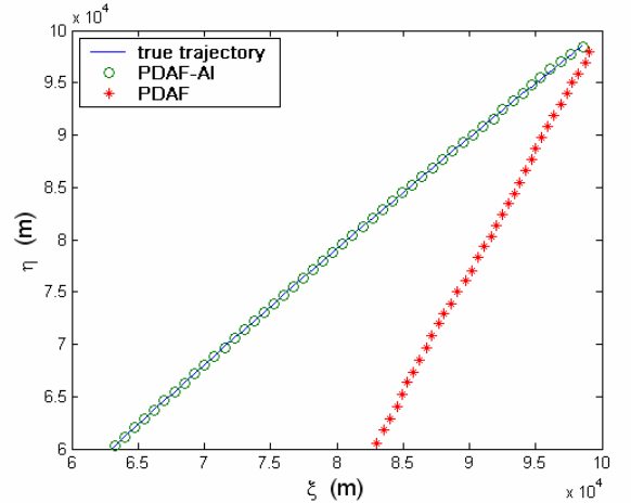
Figure 4. Example of Track with \rho = 10 dB, Clutter Density \lambda = 5 \times 10^{-6} m -2 , Number of Sensors: 1.
