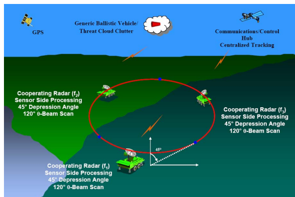
Figure 1. Ground-Based Multi-Radar Target Detection/Tracking.
