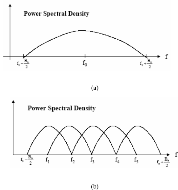
Figure 2. PSD of (a) each CDMA DSSS system and (b) sub-division of original frequency band.
