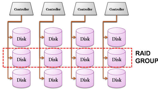
Fig. 2. Orthogonal RAID that can survive controller failure.
