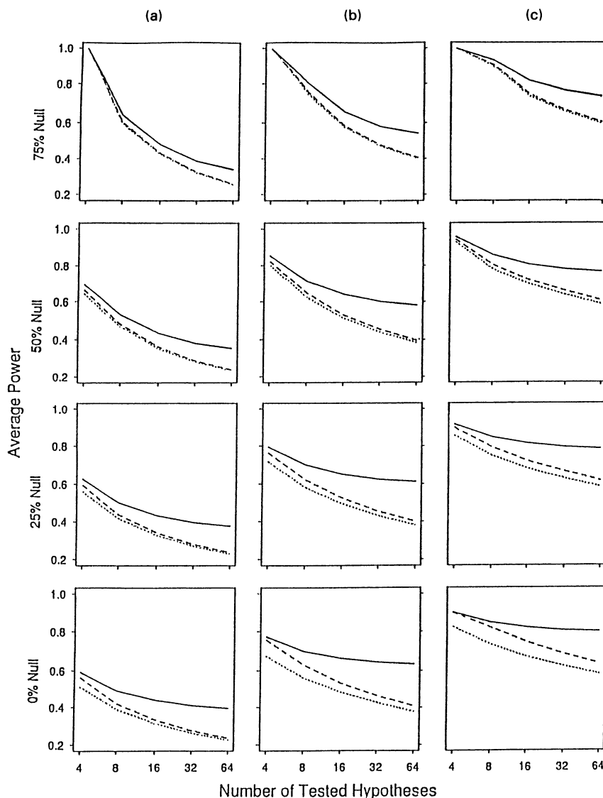
Fig. 1. Simulation-based estimates of the average power (the proportion of the false null hypotheses which are correctly rejected) for two FWER controlling methods, the Bonferroni ( \cdots\cdots ) and Hochberg's (1988) ( -\cdots- ) methods, and the FDR controlling procedure ( -\text{---} ): (a) decreasing; (b) equally spread; (c) increasing
