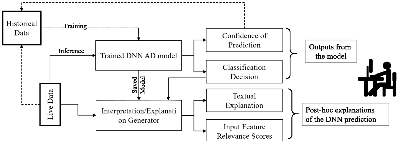
Figure 1: The Presented framework for Explainable DNN based Anomaly detection. The decision maker is the human operator. The operator gets the DNN predictions and the justifications.
