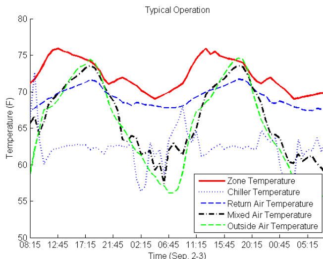
Fig. 7 Typical operation characteristics of the selected office room for a 48 hour period
