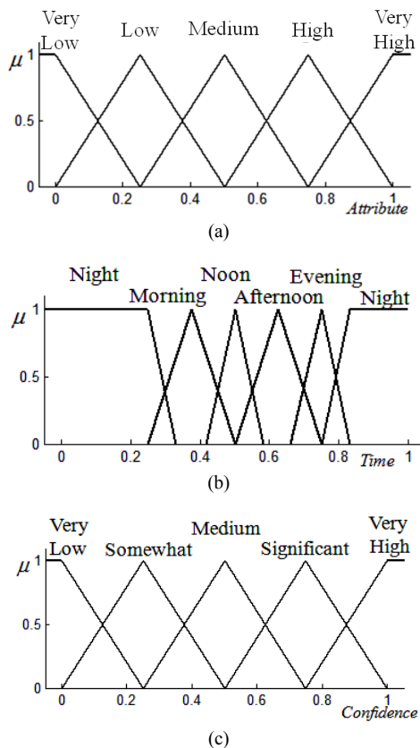
Fig. 3 Linguistic labels for sensor input (a), for time attribute (b), and for anomaly confidence (c).
