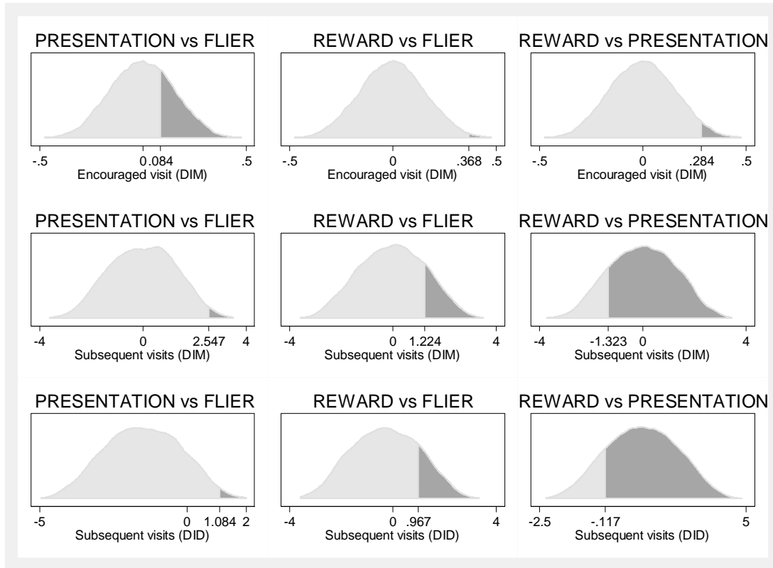
Figure 1 – The randomization distributions of average treatment effects for the sharp null hypothesis H_0: Y_k(f) = Y_k(p) = Y_k(r) for all classes
