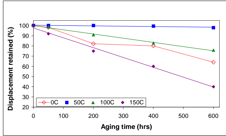
FIG. 8. Isothermal aging.
