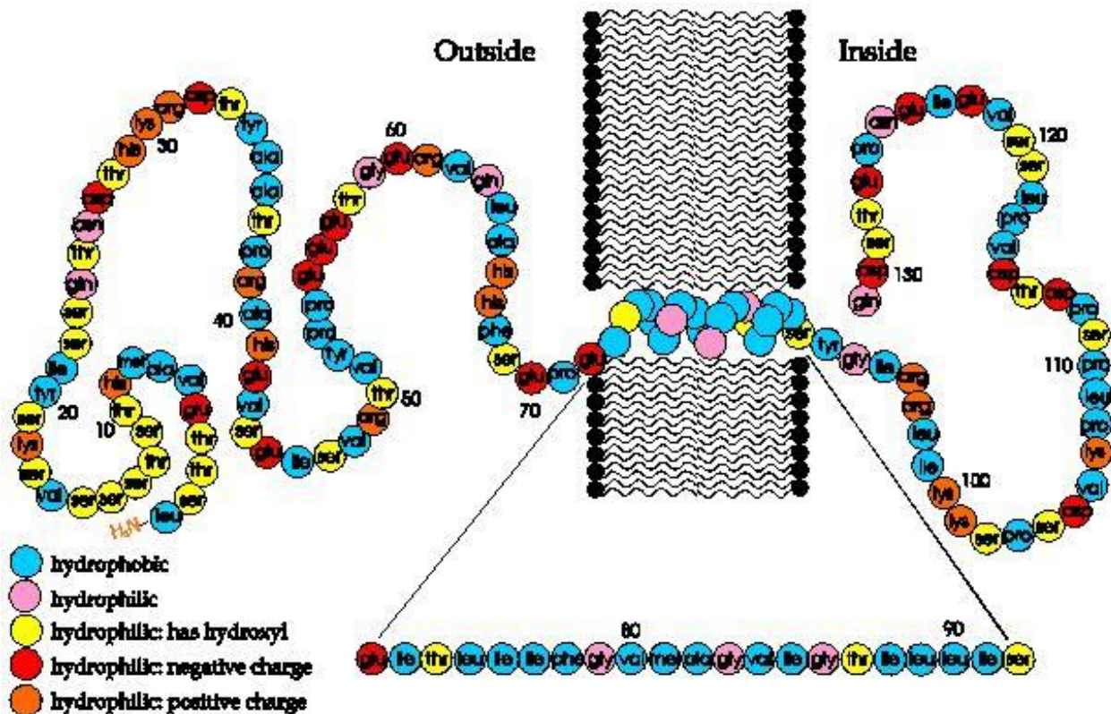
Figure 5. Primary structure of glycoprotein A. Amino acid sequence of one polypeptide of glycoprotein A. Amino acids are colored to show different chemical properties. Note that the charged amino acids all lie not in the membrane but either inside or outside the red blood cell, as do most of the other hydrophilic amino acids. Many of the hydroxylated amino acids on the outside of the cell are also charged, owing to negatively charged sugars (not shown) attached to the amino acids after the protein is made. In contrast, the portion of the protein that spans the membrane consists of amino acids that are predominantly hydrophobic (see also inset at bottom of the figure). These 19 amino acids form an alpha-helix. The regions on both sides of the membrane also have secondary and tertiary structures, not shown in this cartoon. Finally, glycoprotein A has a quaternary structure: in nature (but not in this cartoon) it is a dimer consisting of two identical polypeptide chains associated with one another.
