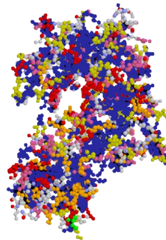
Fig. 2: Three dimensional representation of the enzyme hexokinase. Each ball represents one amino acid out of a total of 457. Blue amino acids are hydrophobic, red negatively charged, orange positively charged, yellow and pink uncharged but hydrophilic. The identities of grey amino acids are unknown. Note the hole in the central part of the protein, where glucose binds.
