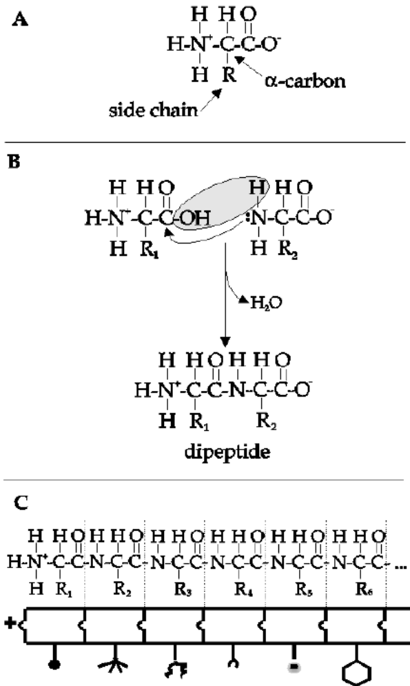
Figure 1. Protein as a polymer of alpha-amino acids. 1A. Structure of alpha-amino acid. "R" represents side group, as shown in Figure 2. 1B. Formation of dipeptide by joining two amino acids. 1C. Polypeptide chain composed of linked amino acids. The shapes represent the different R-groups, each with its own chemical properties.
