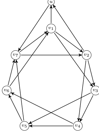
Figure 6: The orientation for Lemma 17 with n = 7 .
