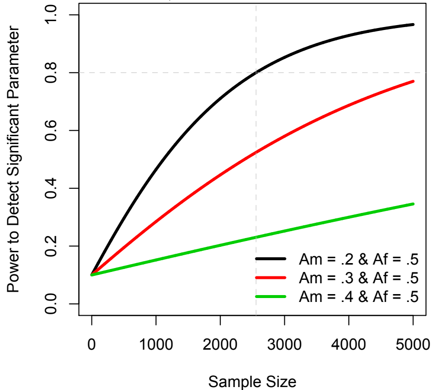
Quantitative Sex Limitation
