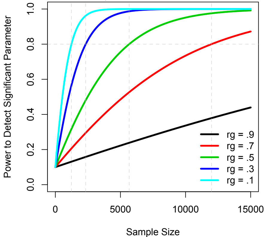
Qualitative Sex Limitation
