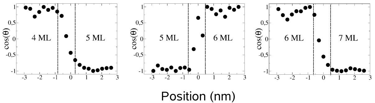
Figure 4. Cosine of the angle of the magnetic surface moments with respect to the bulk obtained in the theoretical calculations shown in Fig. 3 for 4-5, 5-6 and 6-7 ML. Vertical dashed lines specify the size of the domain wall in each case.
