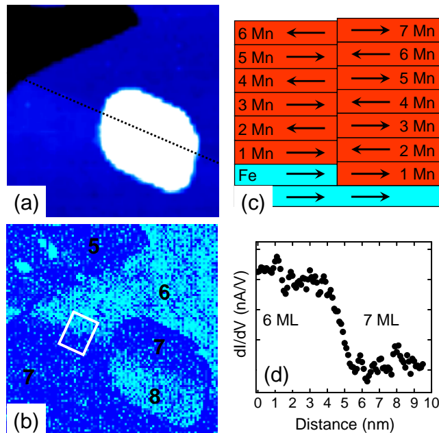
Figure 1. (color online) (a) STM image after deposition of 5 Mn ML's ( 70 \times 70 \text{ nm}^2 ). The dotted line marks the position of the hidden step. (b) dI/dV map taken at +0.2 \text{ V} . The numbers indicate the Mn local thickness. (c) Model of the Mn structure around the hidden step. (d) Average experimental profile across the hidden step measured inside the white box shown in (b).
