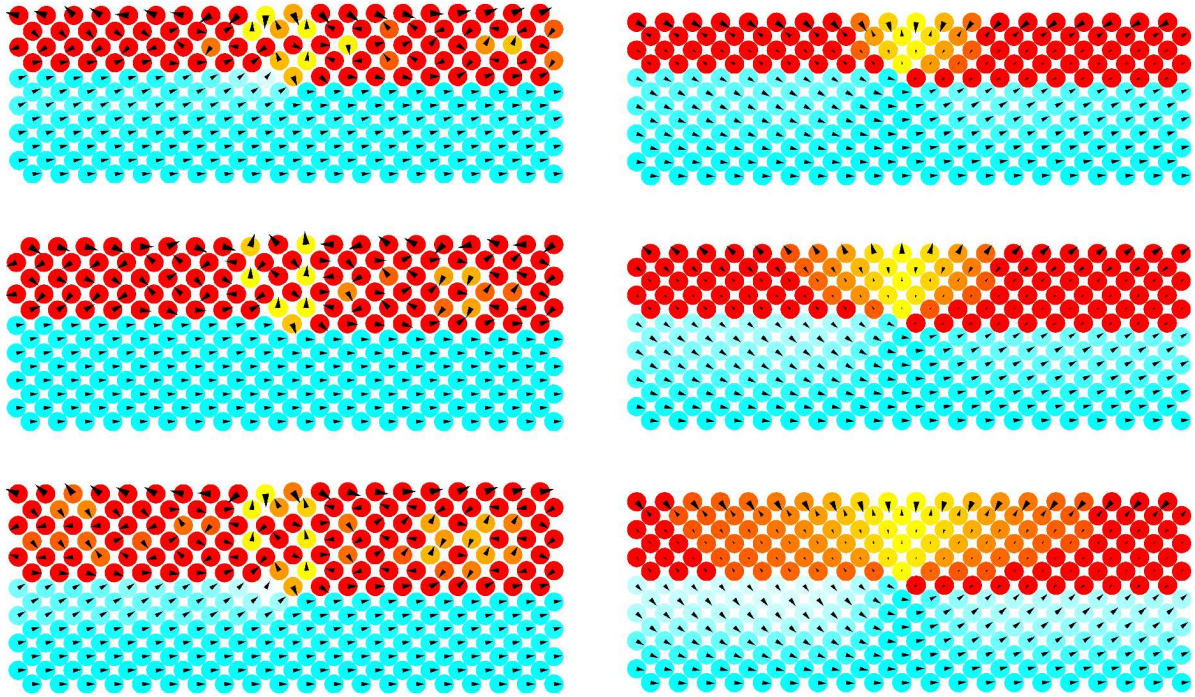
Figure 3. (color online) Result of the calculation performed for 4-5, 5-6 and 6-7 monolayers of Mn (left panel) and Cr (right panel) supported on an Fe(001) substrate with a monoatomic step (only a portion of the calculated systems is represented). The arrows indicates the orientation of the individual magnetic moment and its size is proportional to absolute value of the local magnetic moment (average values of the magnetic moments far from the step: \mu_{Fe}^{bulk} = 2.32\mu_B , \mu_{Mn}^{surf} = 3.84\mu_B , \mu_{Cr}^{surf} = 3.07\mu_B , \mu_{Mn}^{inter} = 2.85\mu_B , \mu_{Cr}^{inter} = 1.13\mu_B ). The color of the circles is given by the absolute value of the cosine of the angle of the magnetic moment. For Mn and Cr red means a LAF arrangement and yellow indicates the magnetic moment at 90^\circ . For the Fe(001) substrate the blue color indicates a ferromagnetic arrangement and light blue a deviation from that.
