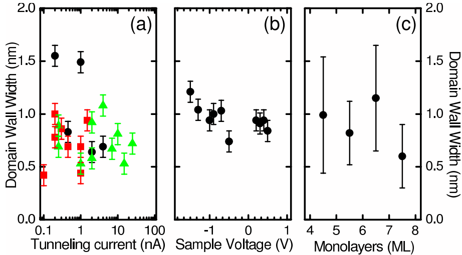
Figure 2. (color online)(a) Shows the domain wall width versus the tunneling current (tip-sample separation). Black dots, green triangles and red squares were obtained at a voltage set point of V_s = +1.5 V, V_s = +0.8 V, and V_s = -1.0 V, respectively. (b) Shows the domain wall width versus bias voltage. The experiments were done on hidden steps between 4-5 ML and 6-7 ML. (c) Domain wall width versus Mn thickness.
