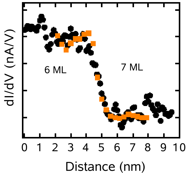
Figure 5. (color online) (black dots) Average experimental profile across the hidden step measured inside the white box shown in Fig. 1(b). (orange squares) Cosine of the angle of the magnetic surface moments with respect to the bulk obtained in the theoretical calculation shown in Fig. 3 for 6-7 ML.
