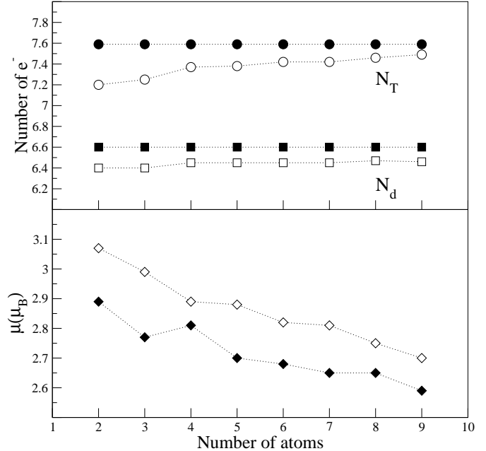
Fig. 1. Number of electrons (upper panel) and magnetic moment (lower panel) per atom of \text{Fe}_n clusters ( n = 2-9 ) supported on Ni(001), as function of n . Filled symbols correspond to LCNA calculations and open circles to GCNA calculations. In the upper panel, circles represent total occupations and squares d occupations. Lines joining points and merely visual aids.
